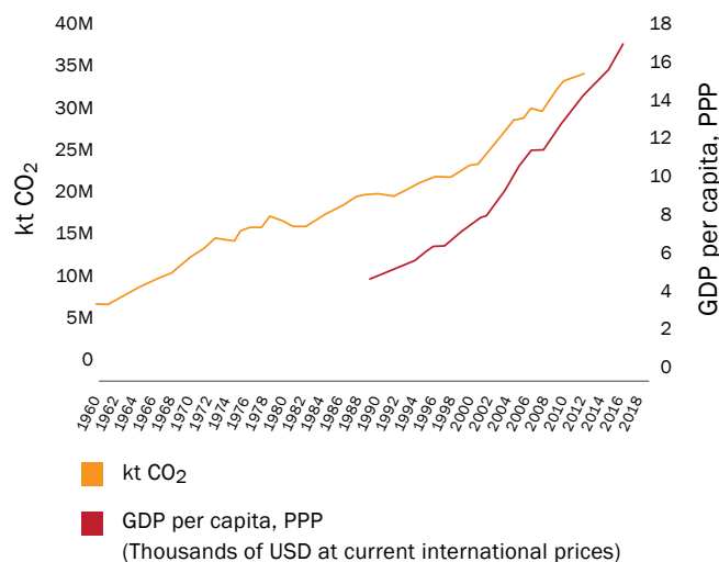
Figure 2: Emissions and GDP per capita
