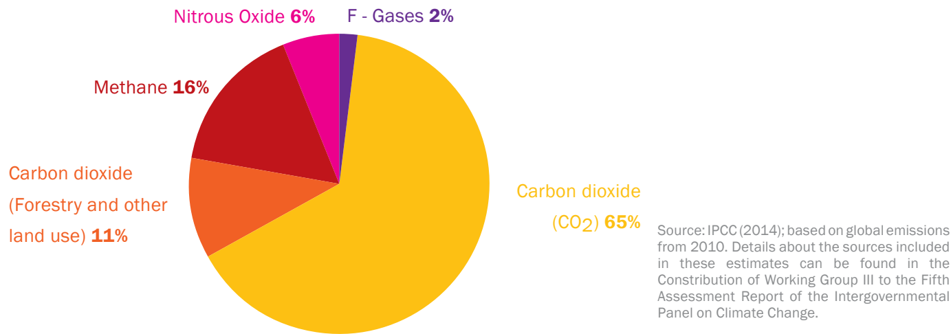
Figure 3: Carbon emissions by sources
