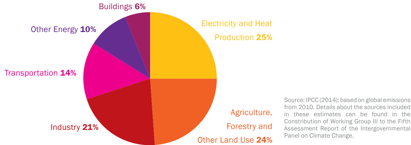
Figure 4: Carbon emissions by sectors
