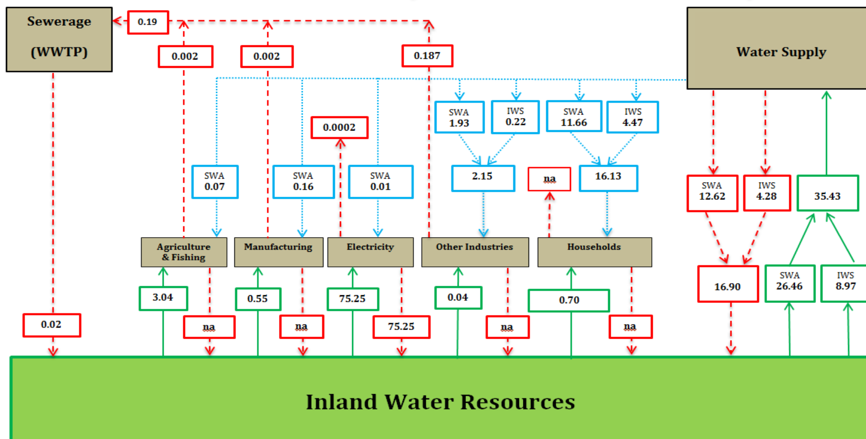
Fig. 1: Major Water Flows in Samoa 2014-15 (millions m 3 )
