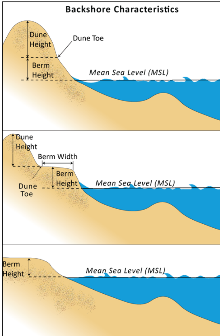
Figure 7.9: Definition of Berm Height, Berm Width and Dune Height at a typical sandy beach.
