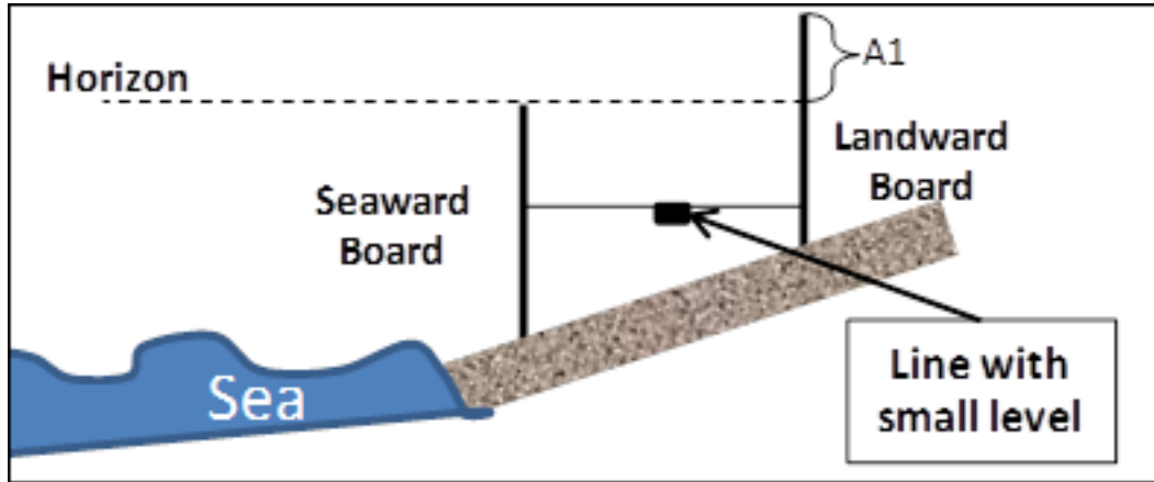
Figure 7.21: Same as previous figure. Find distance A1 from top of board to eye such that eye, top of board 2 and horizon are aligned. Line must be horizontal.
