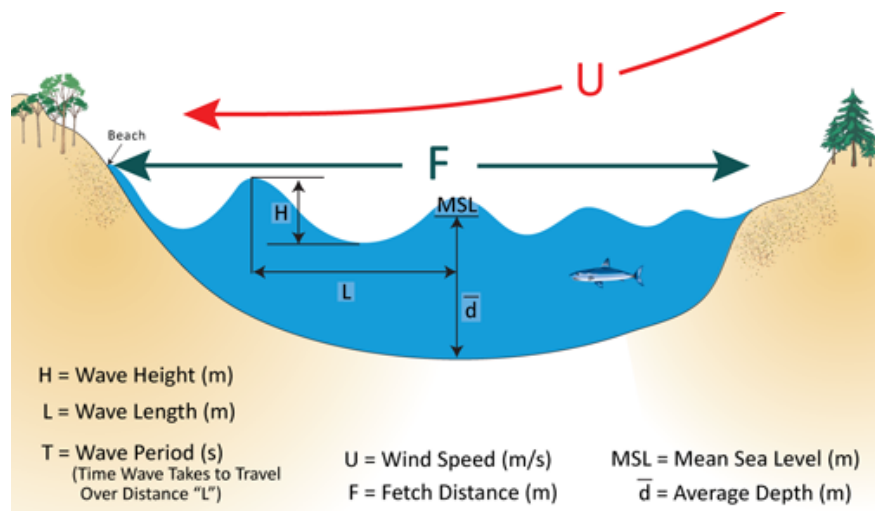
Figure 7.4: Definition of various coastal engineering terms used in the model.
