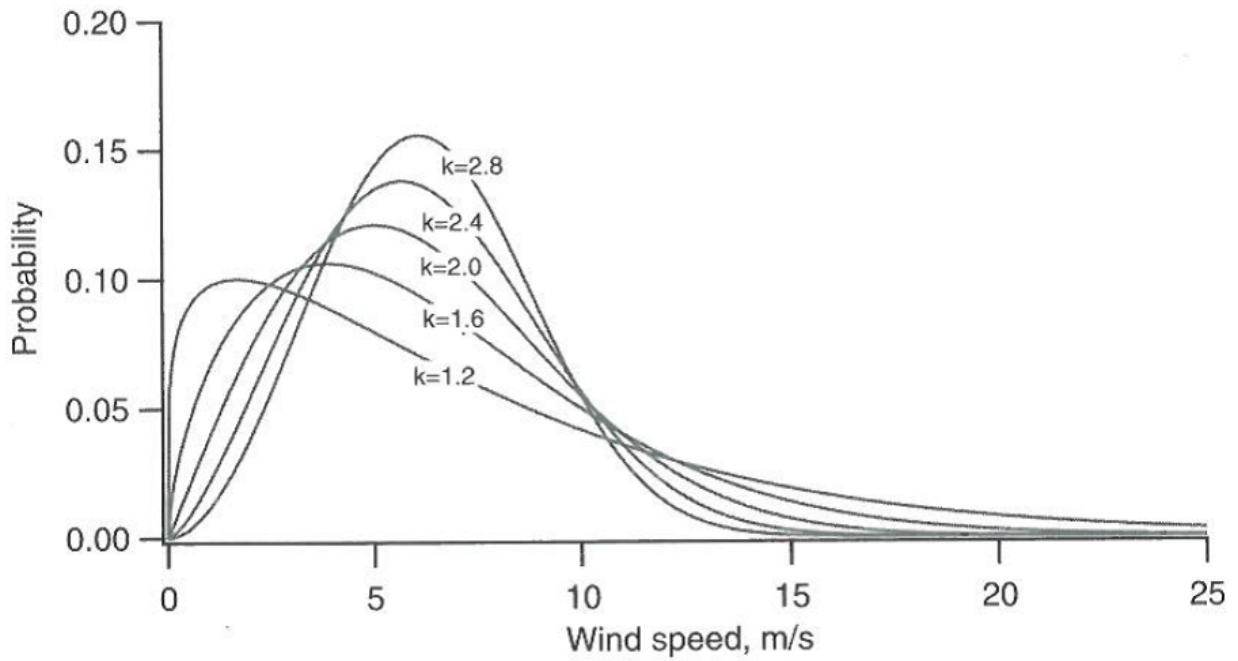
Figure 5.1: Example of Weibull probability density function with various shape factors ( k ), where mean wind velocity = 6\text{m.s}^{-1} (Manwell et al., 2009).
