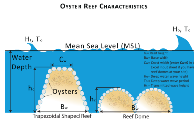
Figure 7.19: Depiction of typical shapes of oyster reefs, along with definition of terms used in the input Excel sheet.
