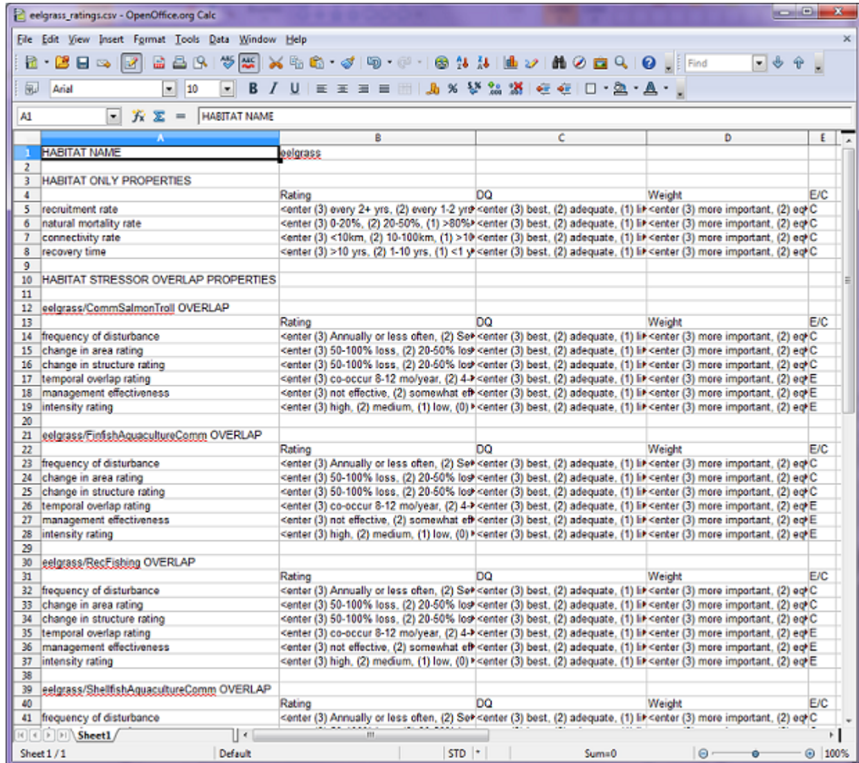
Figure 11.4: Upon initial creation, CSVs will contain no ratings, only guidance for known criteria on a scale of 0-3. However, users should feel free to fill in ratings on a different scale if there is significant reviewed data, but should be sure to be consistent on scale across ALL CSVs.
