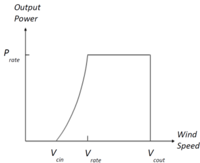
Figure 5.4: Output power (P) curve of a wind turbine (pitch control type) as a function of wind speed (V) (Modified from Fig.1 in Pallabazzer 2003)
