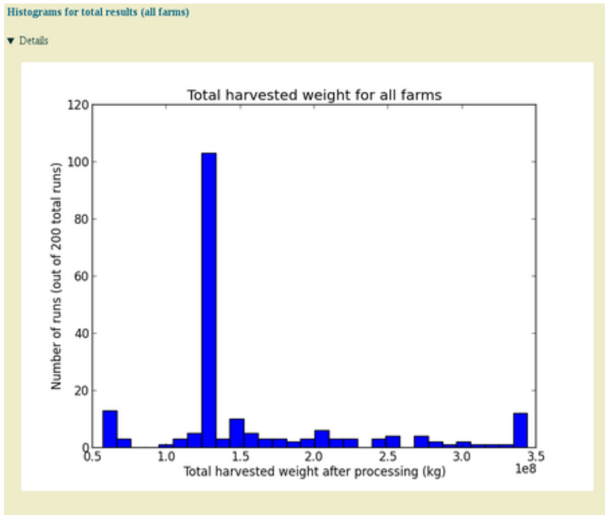
Figure 8.4: Sample histogram in the uncertainty analysis section of HTML output
