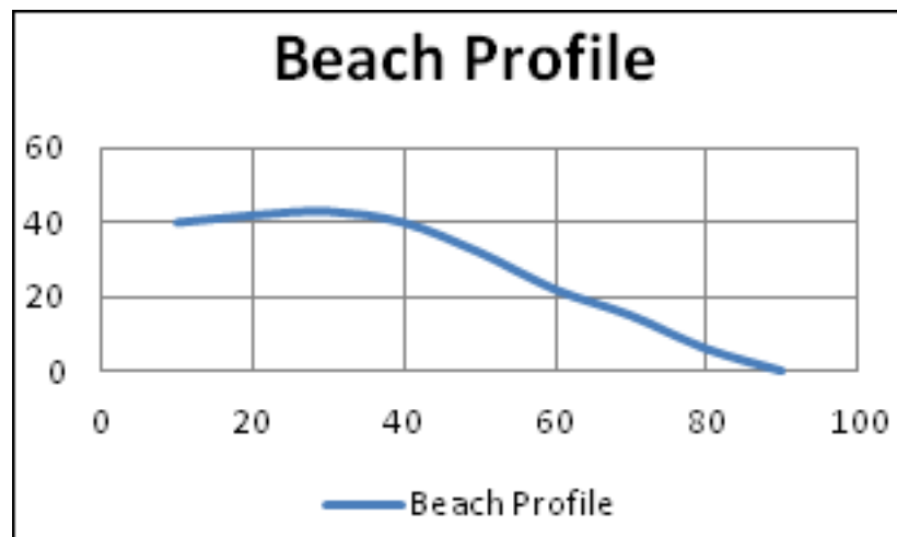
Figure 7.23: Example beach profile measured with Emery Board. Zero is last point measured.
