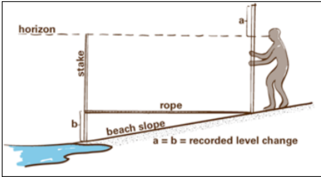
Figure 7.20: Illustration of the Emery Board technique
