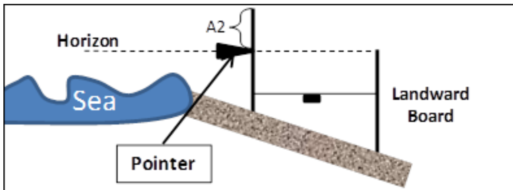
Figure 7.22: Same as two previous figures. Find distance A2 from top of board to pointer such that eye at top of board 1, pointer and horizon are aligned. Line must be horizontal.
