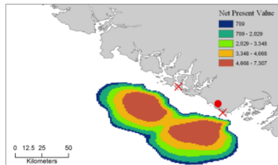
Figure 4.6: Net present value (thousand $) over a 25-yr life-span, using $500,000 per km for the cost of underwater transmission cables. Two underwater cable landing points are located in Tofino and Ucluelet (x) and power grid connection point is located in Ucluelet (o). Each of the WEC facilities is composed of 28 Pelamis devices. The price of electricity is set at 20 cents per kW.
