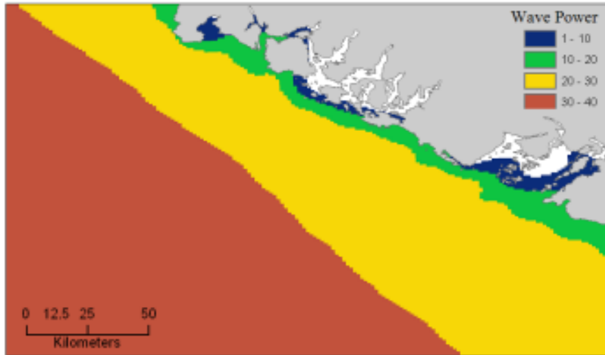
Figure 4.3: Wave power potential (kW/m) in the west coast of Vancouver Island.
