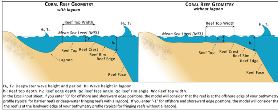
Figure 7.17: Profiles of coral reefs in the presence or absence of a lagoon, along with definition of the terms used in the Excel input sheet.
