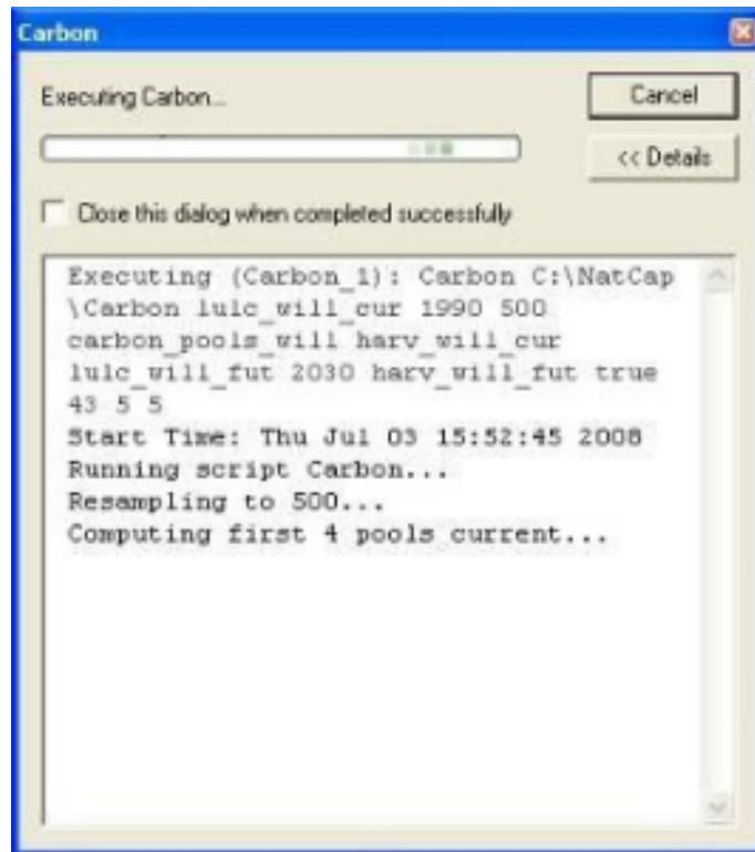
Figure 3.4: Progress dialog
