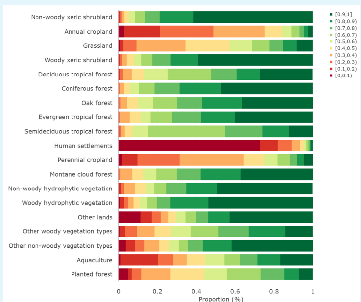
Figure 5: Proportional distribution of aggregated ecosystem integrity according to CONAFOR-IPCC-N3 categories for 2018
