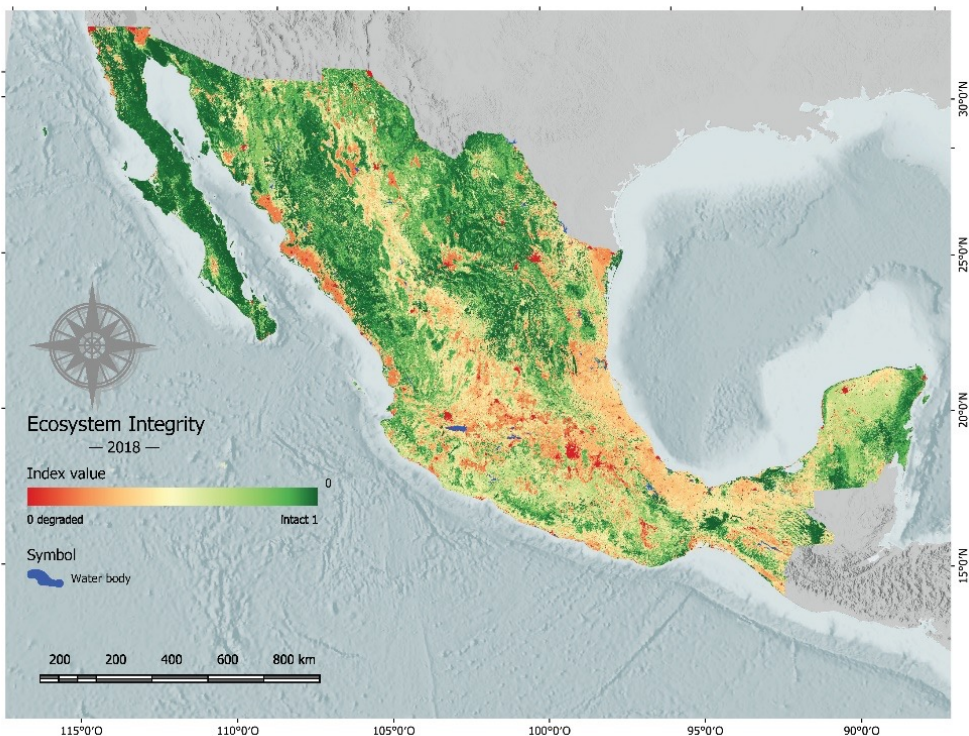
Figure 4: Ecosystem Integrity Index for the terrestrial ecosystems of Mexico in 2018 (250 X 250 m or 6.25 ha grids).
